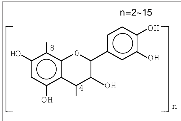
Figure 2. Chemical structure of procyanidins.
